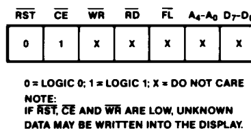
Figure 7. Logic Levels to Reset the Display.
