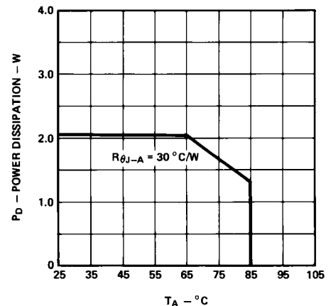
Figure 8. Maximum Power Dissipation vs. Ambient Temperature Derating Based on T_{j\text{MAX}} = 125^\circ\text{C} .
