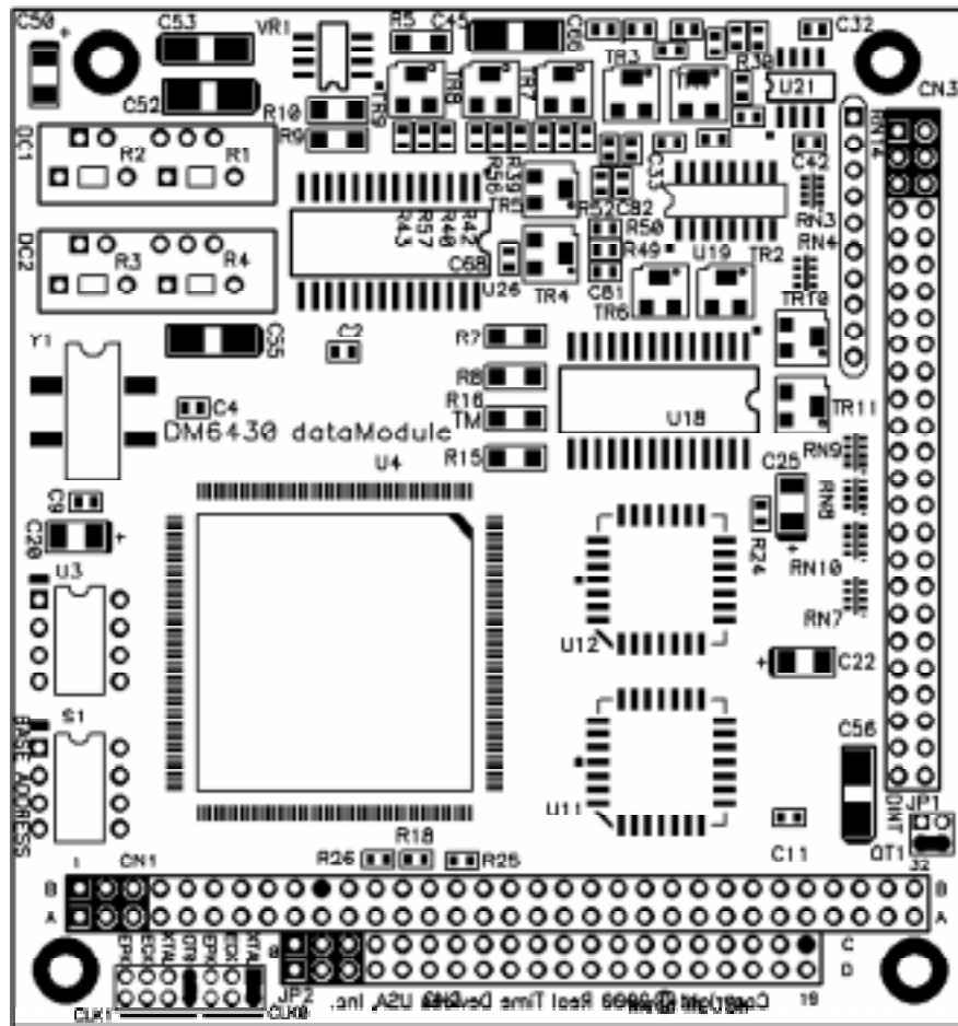
Fig. 12-1 — Board Layout
