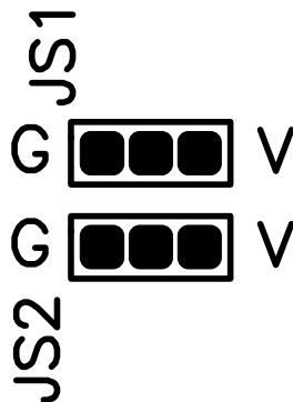
Fig. 1-8 — Ports 0 and 1 Pull-up/Pull-down Resistor Connections
