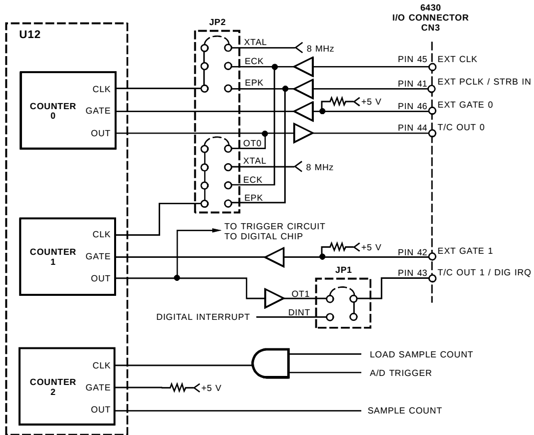
Fig. 1-4 — User TC Circuit Diagram
