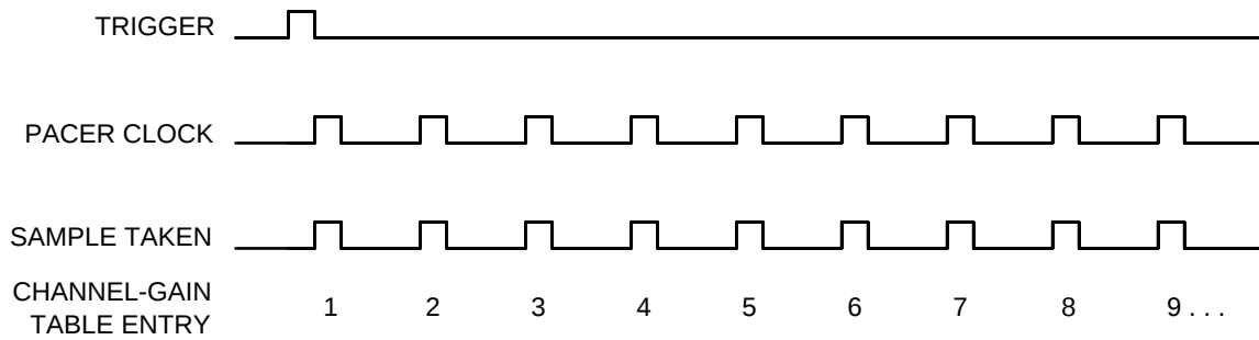
Fig. 5-7 — Timing Diagram, Random Channel Scan
