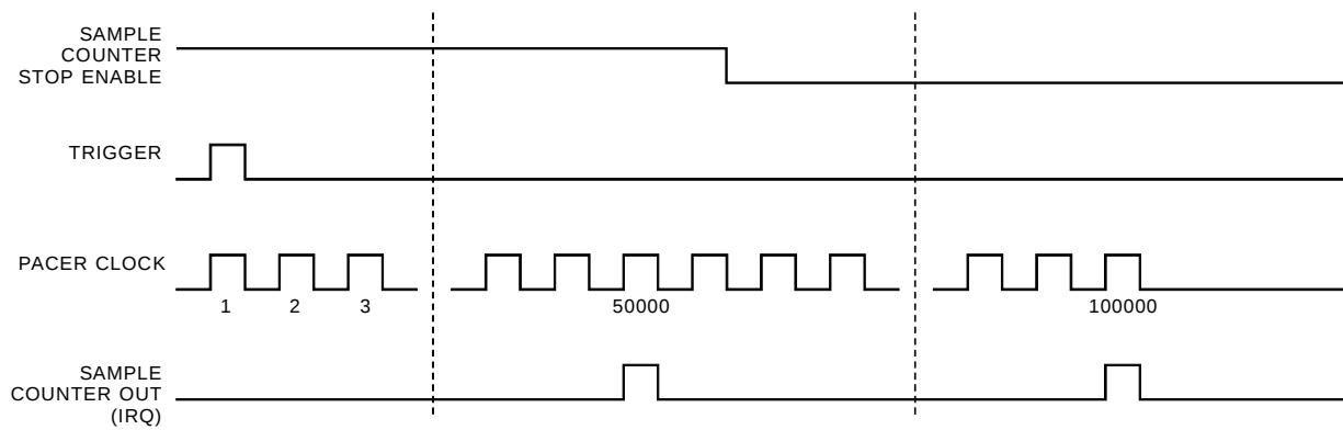
Fig. 5-13 — Timing Diagram for Cycling the Sample Counter
