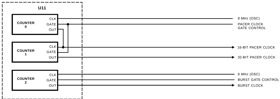
Fig. 3-2 — Clock TC Circuit Block Diagram
