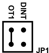
Fig. 1-2 — CN3, Pin 43 Signal Select Jumper, JP1
