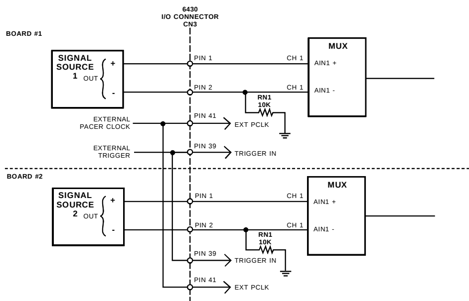
Fig. 2-4 — Two Modules Configured for Simultaneous Sampling
