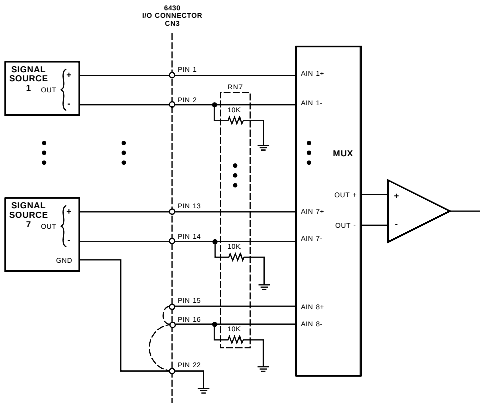
Fig. 2-3 — Differential Input Connections
