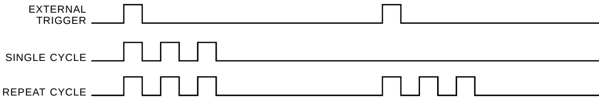
Fig. 5-4 — External Trigger Single Cycle Vs. Repeat Cycle
