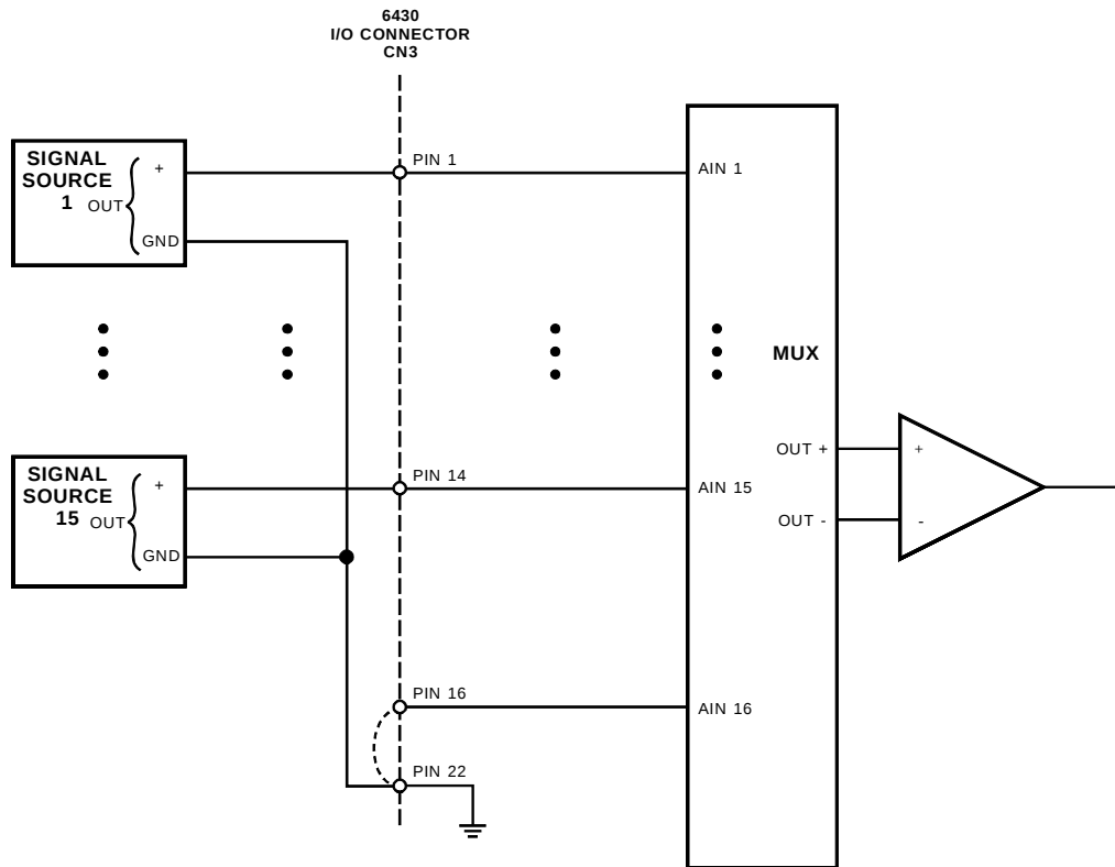
Fig. 2-2 — Single-Ended Input Connections
