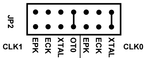
Fig. 1-3 — User TC Clock Sources Jumpers, JP2
