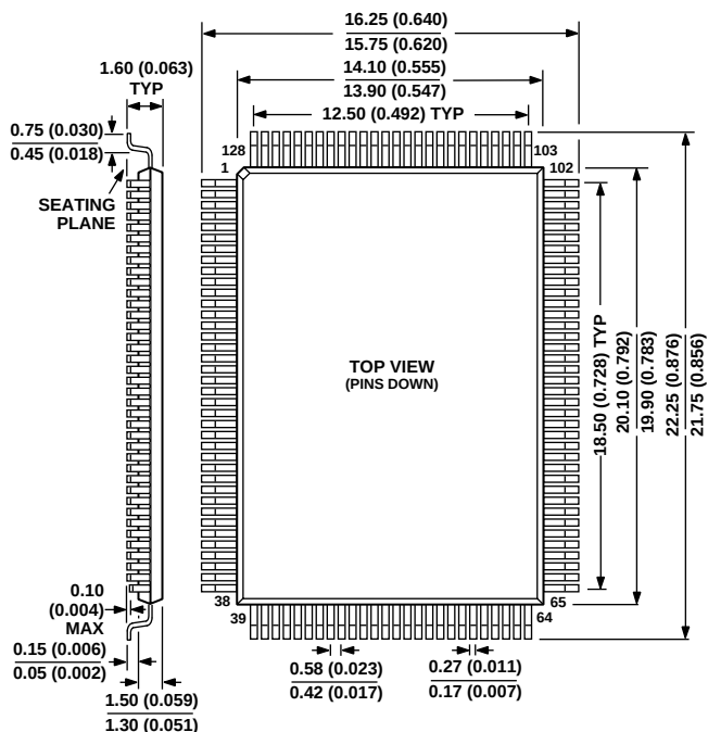
128-Lead Metric Thin Plastic Quad Flatpack (TQFP) (ST-128)
