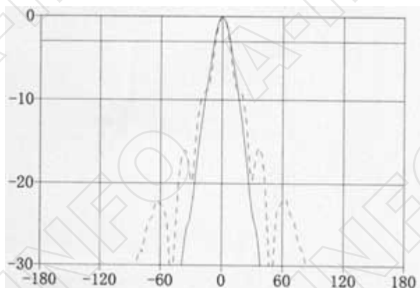
Frequency: 16.5GHz
