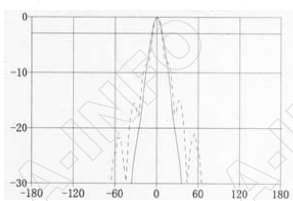
Frequency: 18.0GHz
