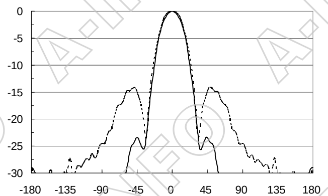
Frequency: 92.5GHz
