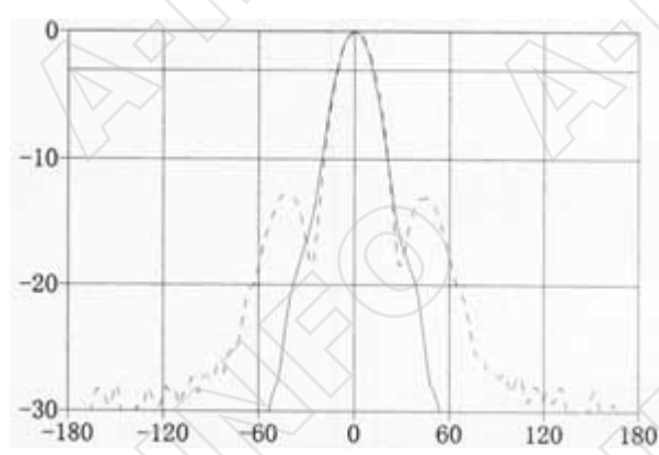
Frequency: 8.50 GHz
