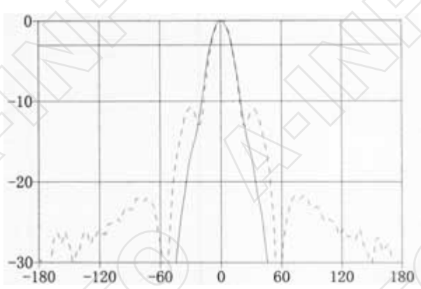
Frequency: 10.00GHz
