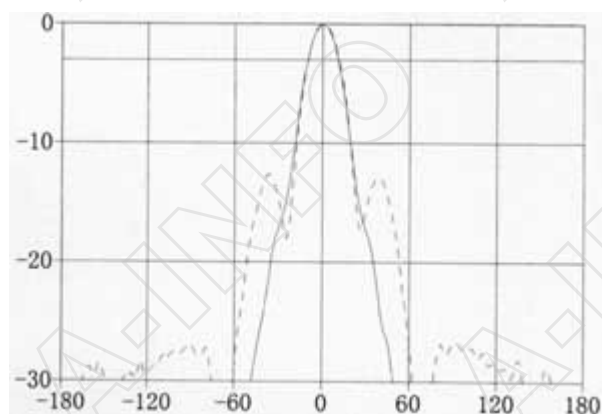
Frequency: 9.50GHz
