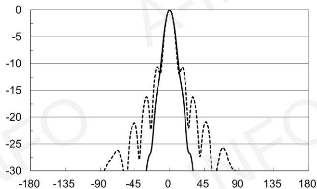
Frequency: 140.0GHz
