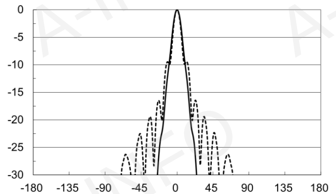
Frequency:180.0GHz
