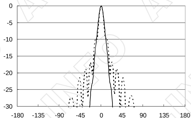
Frequency: 115.0GHz
