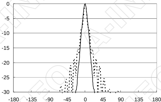
Frequency: 140.0GHz
