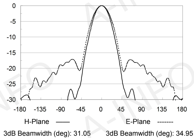
Frequency: 33.0GHz
