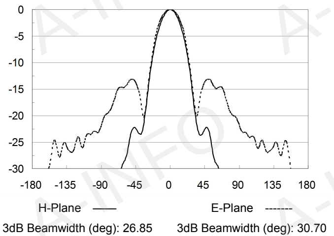
Frequency: 41.5GHz
