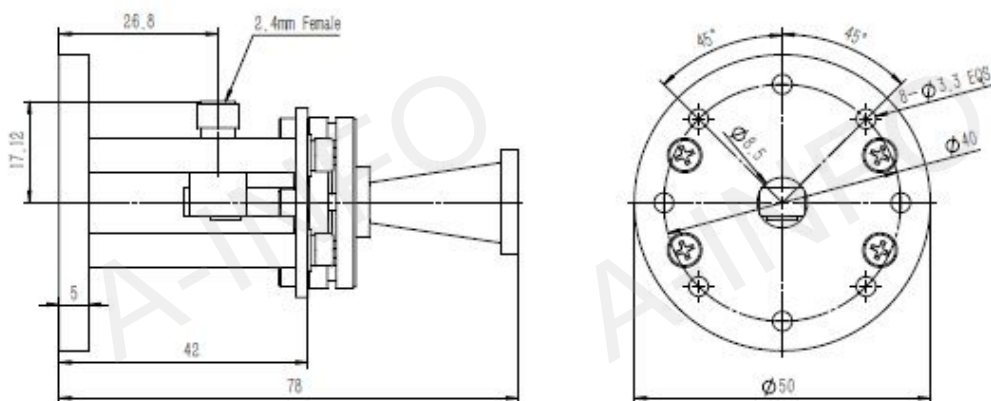
C Type(with Round Mounting Bracket and Radome)
