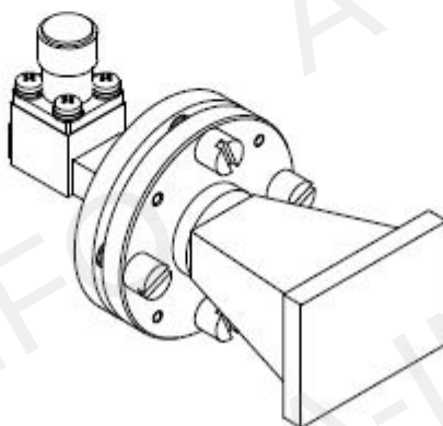
C Type(with Round Mounting Bracket and Radome)
