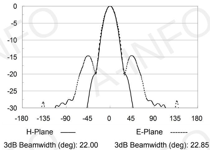
Frequency: 50.0GHz
