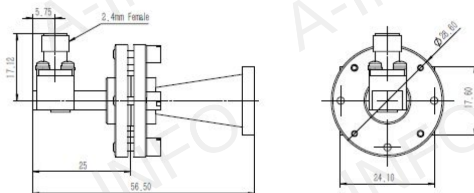
C Type(with Radome)
