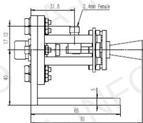
C Type(with L type Mounting Bracket)
