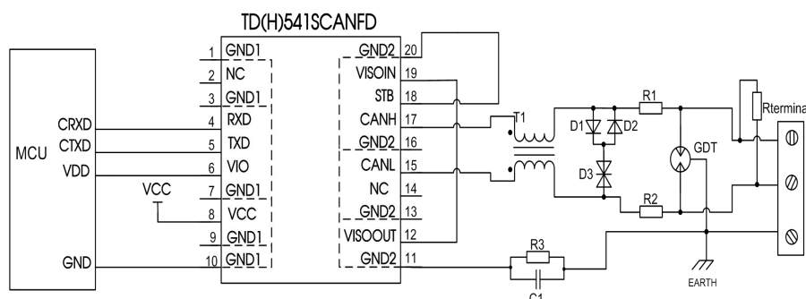
When the module is in normal condition attach STB feet to GND2
