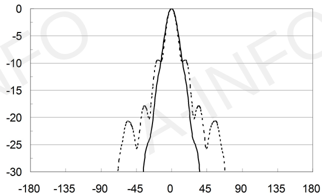
Frequency: 50.0GHz
