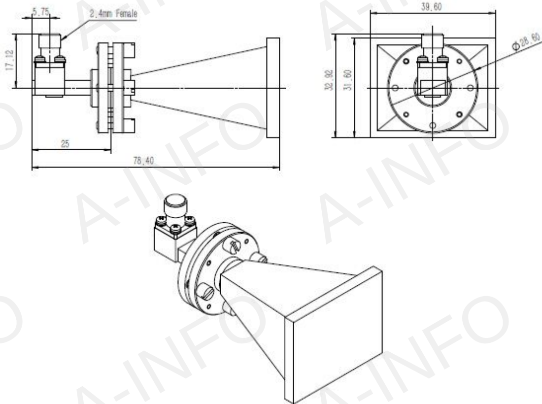
C Type(with Round Mounting Bracket and Radome)
