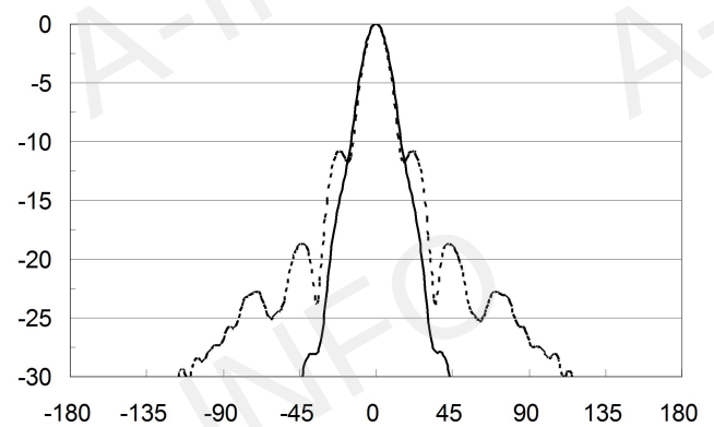
Frequency: 41.5GHz
