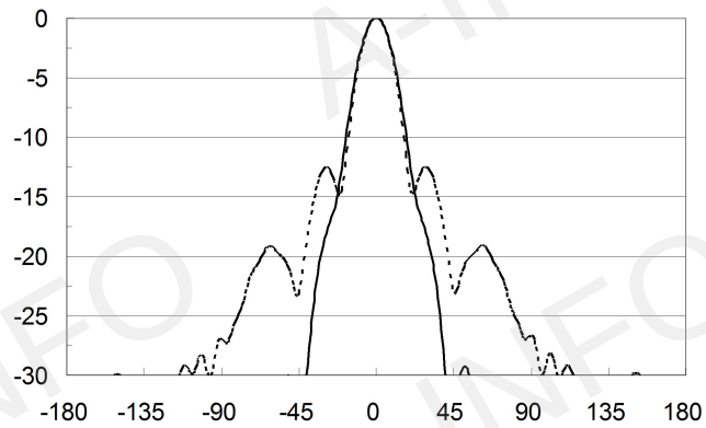
Frequency: 33.0GHz
