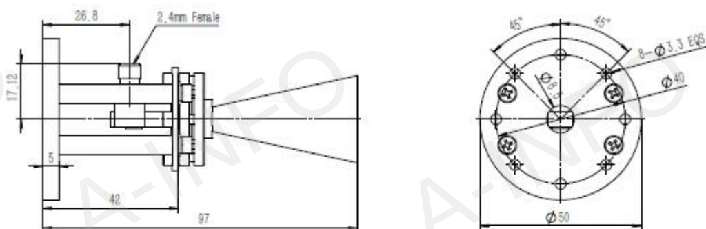
C Type(with Round Mounting Bracket)
