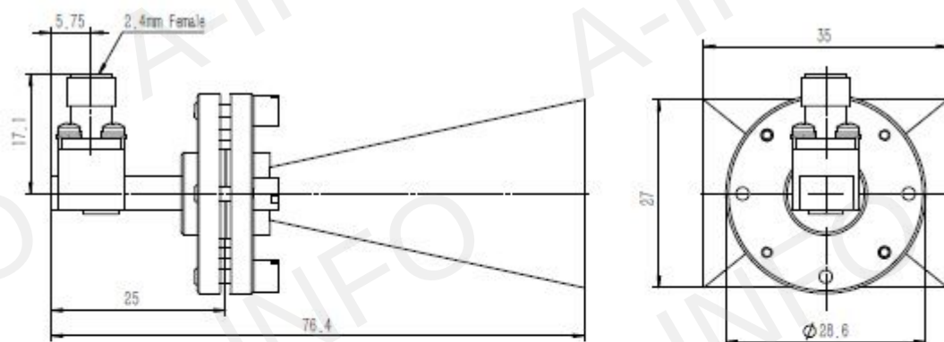
C Type(with 2.4mm Female output)
